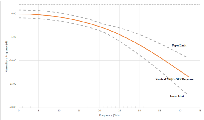
Fourth order Bessel-Thompson frequency response of the DPO70E1 Optical Probe and DPO70000SX ATI channel
