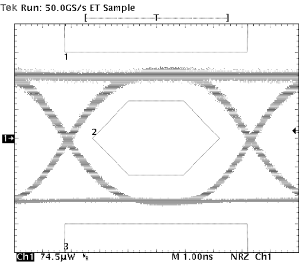
OC-3/STM-1 SONET/SDH Transmitter Eye Pattern Test
