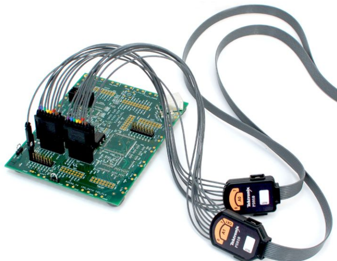
P5910 17-channel general purpose probe
